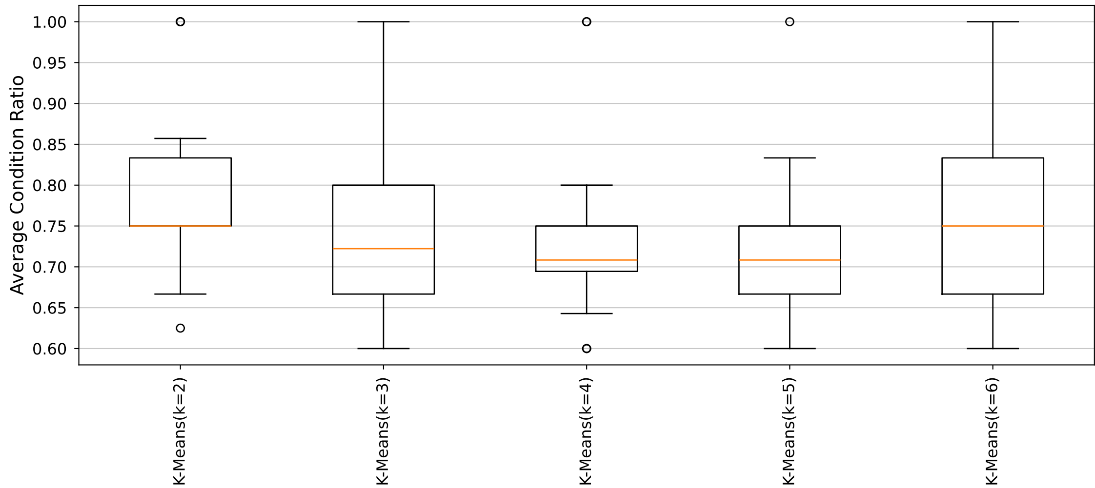
YARA Rules Average Condition Ratio Distribution (Cluster31_Size6 dataset)
